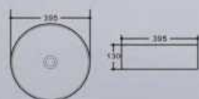
Art Basin Size:395x395x130mm Vareous china Above counter mountings
